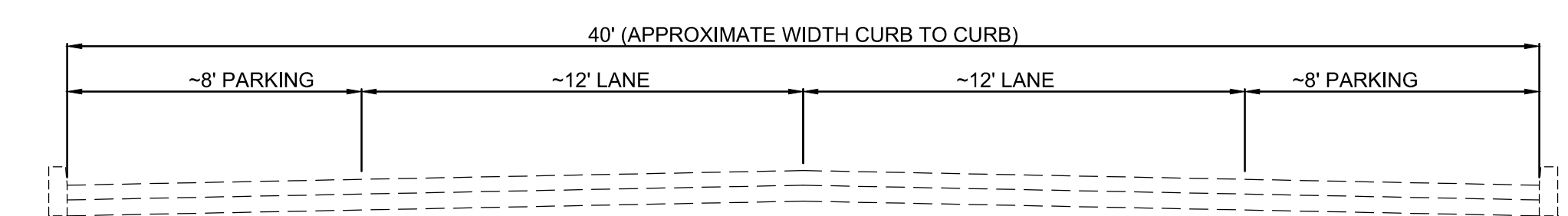
S DIVISION STREET EXISTING SECTION NTS
