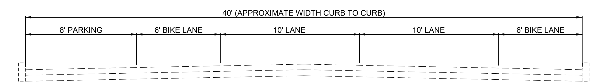
S DIVISION STREET SECTION W/BIKE LANES NTS
