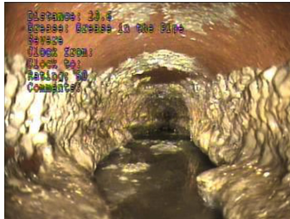
This photo of the inside of a sewer pipe in Walla Walla shows what fat, oil and grease buildup looks like.
